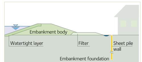
Illustration 4: protection against subsidence
