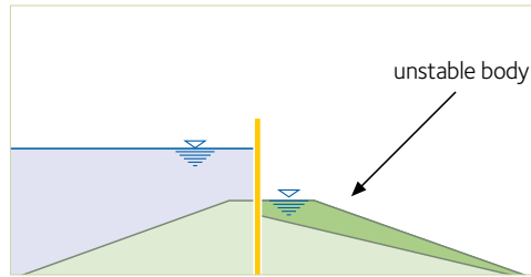
Illustration 4: Rising flood: slip of part of the flooded landward shoulder ( \phi_{\text{wet}} < \phi_{\text{dry}} ).
