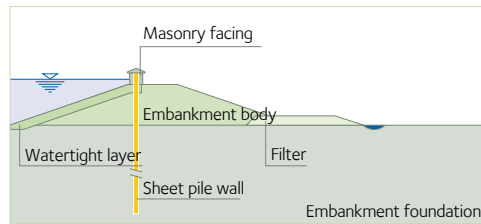
Illustration 2: raised design flood level
