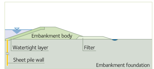
Illustration 3a: stabilization of inner shoulder (protection against scour)
