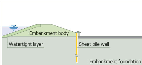
Illustration 3b: stabilization of outer shoulder
