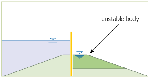
Illustration 3: Rising flood: part of the outer shoulder is at risk of being washed away by overflow.
