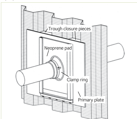
Pipe penetration
