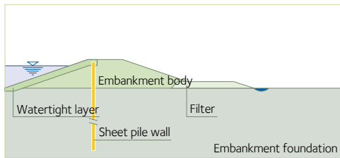
Illustration 1: cutoff
