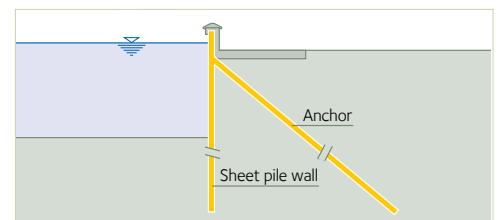
Illustration 5: flood wall
