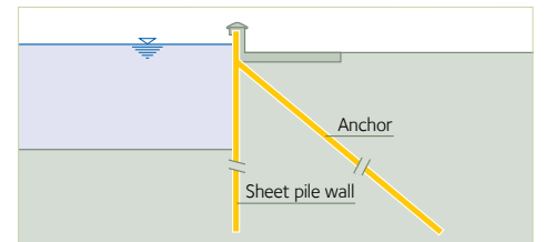
Illustration 5: flood wall
