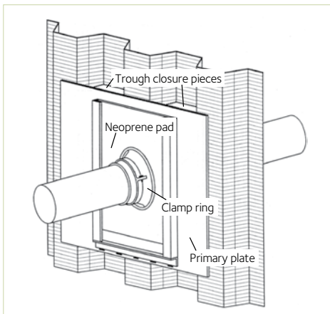
Pipe penetration
