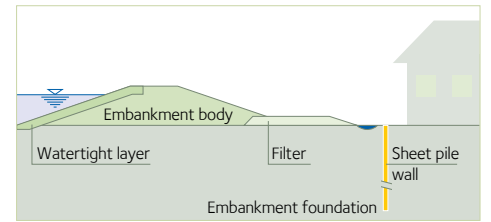
Illustration 4: protection against subsidence
