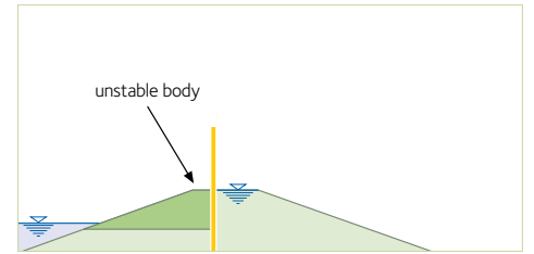
Illustration 5: Receding flood: part of the inner shoulder is at risk of being washed away by much stronger currents during the flood.
