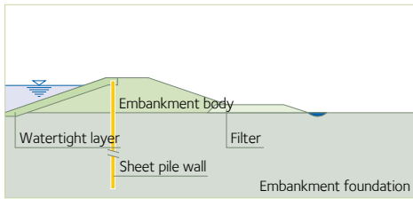
Illustration 1: cut-off
