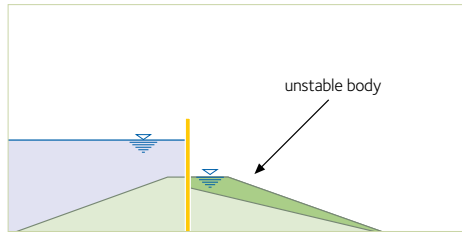
Illustration 4: Rising flood: slip of part of the flooded landward shoulder ( \phi_{\text{wet}} > \phi_{\text{dry}} ).
