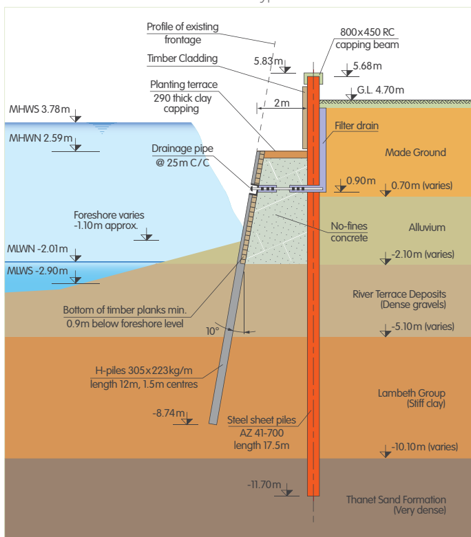
Typical cross section at Hilton's Wharf
