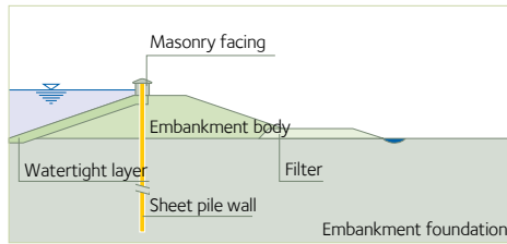
Illustration 2: raised design flood level
