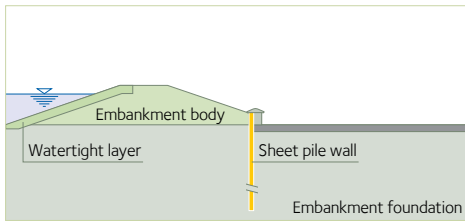
Illustration 3b: stabilization of outer shoulder
