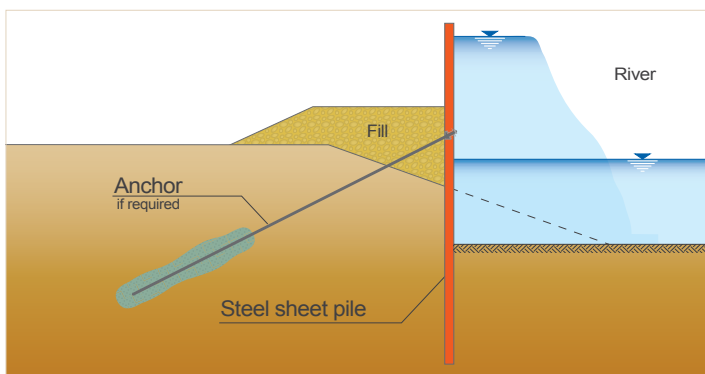
Fig.4 Widening of the river cross-section and flood retaining wall
