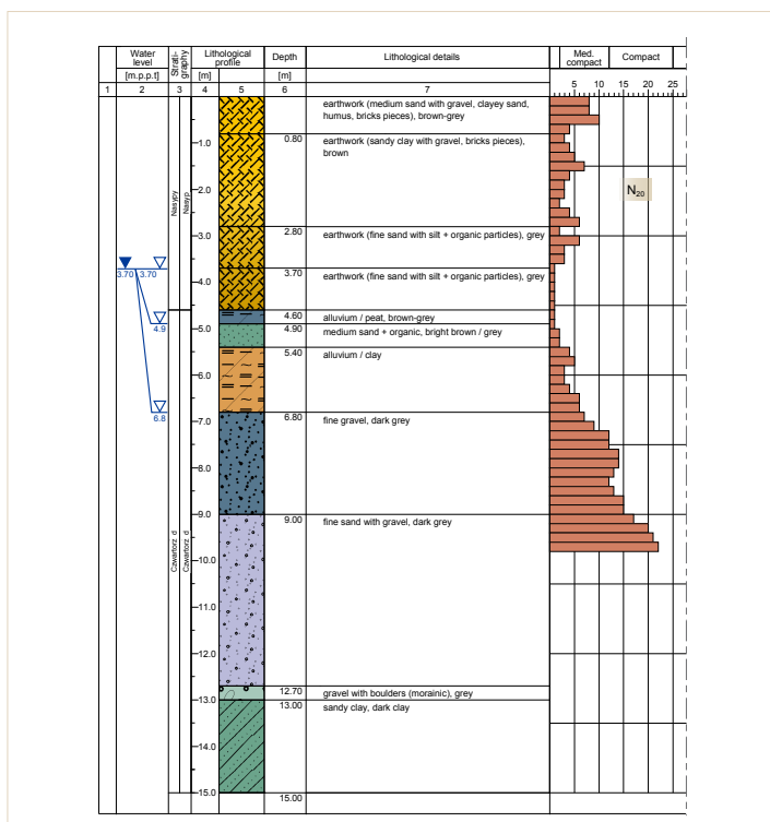
Fig.5 Borelogs
