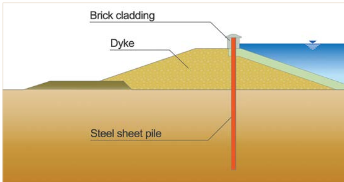
Fig.3 Extension of the flood protection system height with a brick wall cladding
