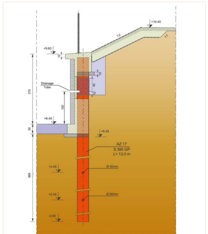
Fig.6 Typical cross-section of a rehabilitated berm of the Radunia Channel (Gdansk)
