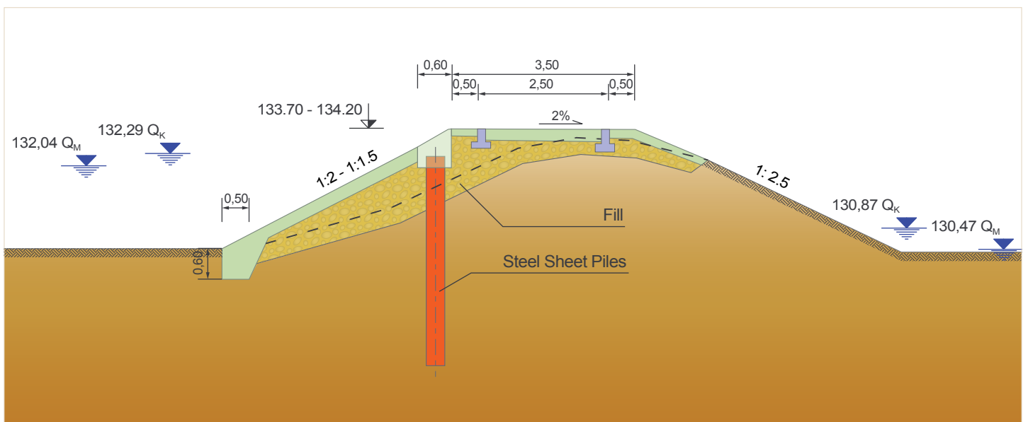
Fig.9 Lipki – Olawa. Typical cross-section
